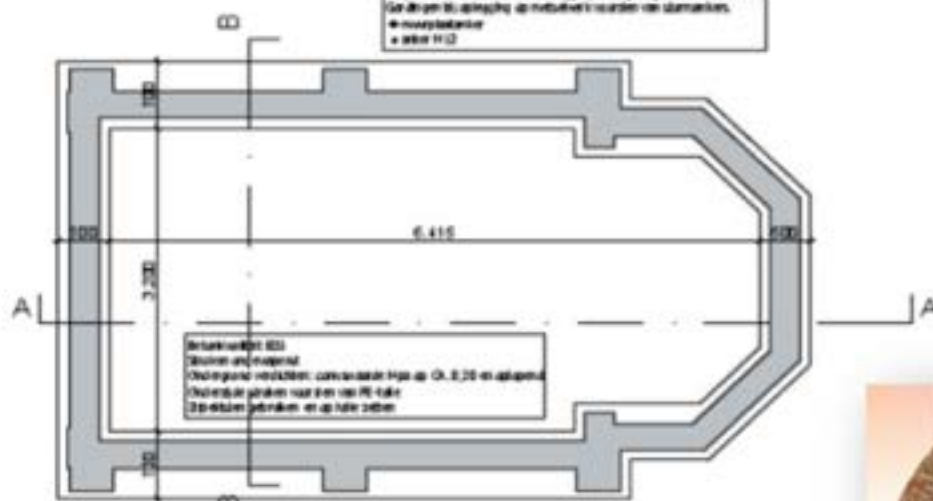
Fundering
